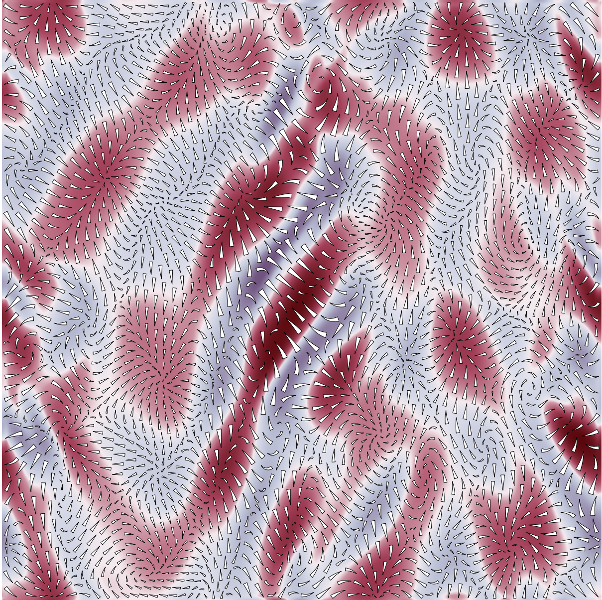
Velocity field in a magnetohydrodynamics simulation illustrating the suppression of turbulence by shearing — vplot 2.0.1
