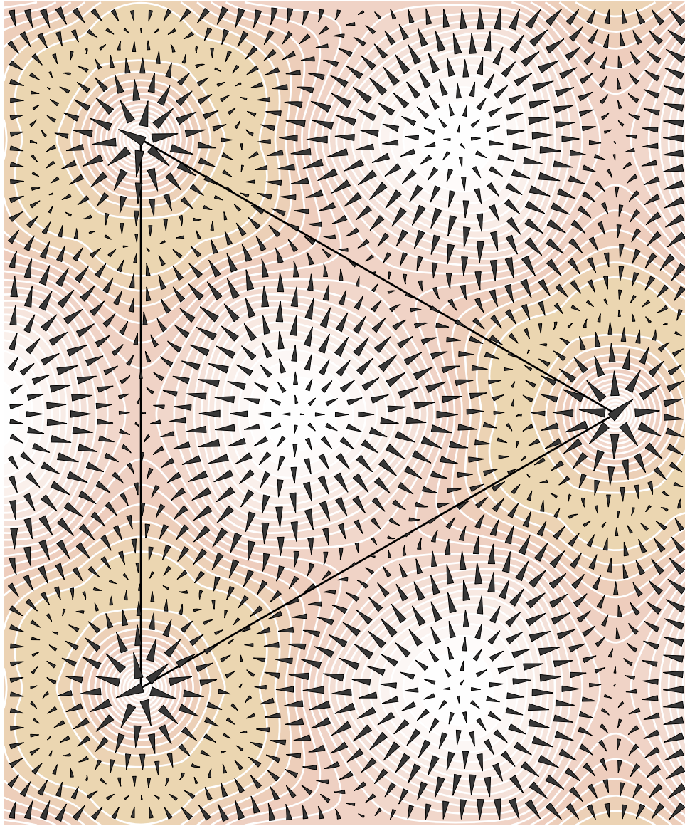
Truncated Lennard-Jones potential given by three discs arranged in a triangle — vplot 2.0.1
