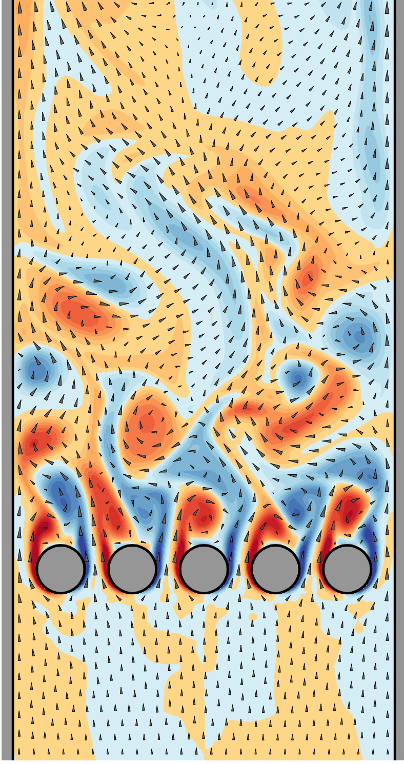
Turbulent flow past a coarse grating — vfplot 1.0.3
