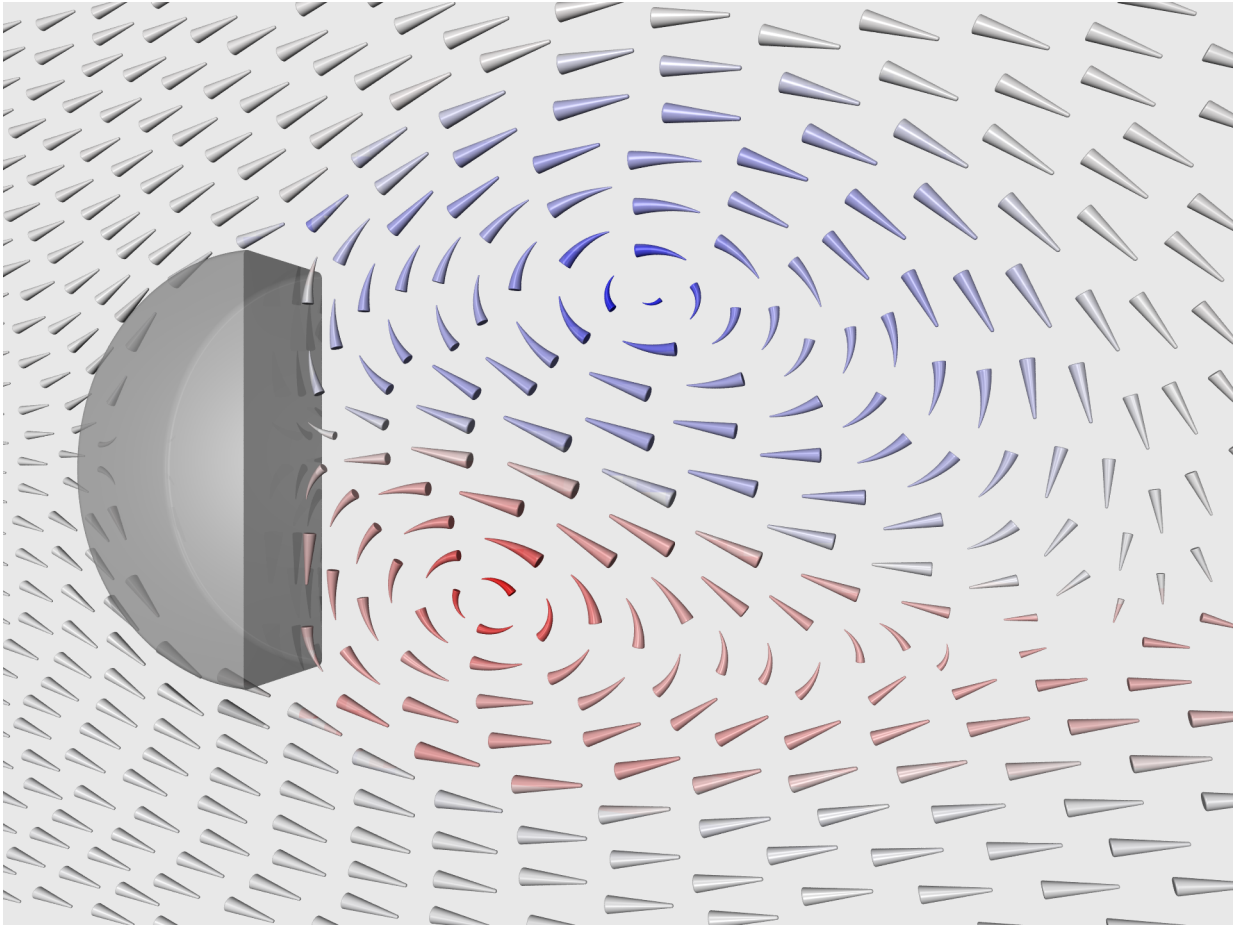
Vortex sheet detachment in flow around a half-cylinder, coloured by vorticity — vfplot 2.0.1, POV-Ray 3.7
