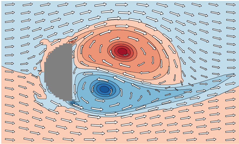
Vortex sheet detachment in flow around a half-cylinder, background is vorticity — vplot 1.0.3
